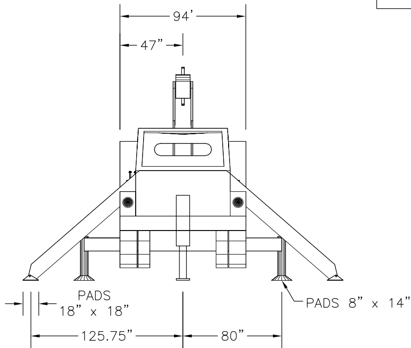
FRONT STABILIZER
