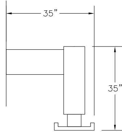
REAR STABILIZER 26" STROKE
